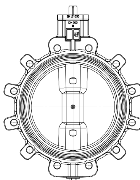
DN250-400
