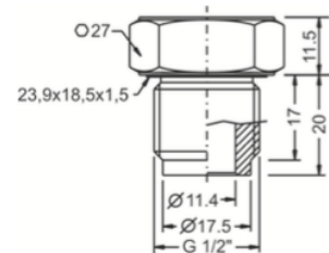
G 1/2" ISO 228-1 – internal bore 11,4mm
