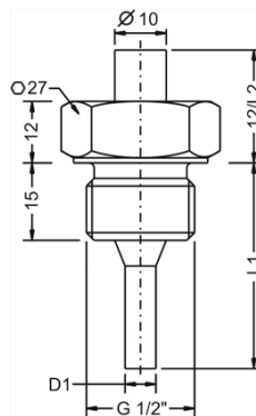
G 1/2"
