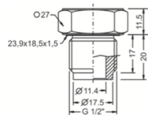
G 1/2" ISO 228-1 – foro interno 11,4mm
